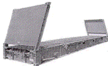
FLAT RACK COLLAPSIBLE 20'
